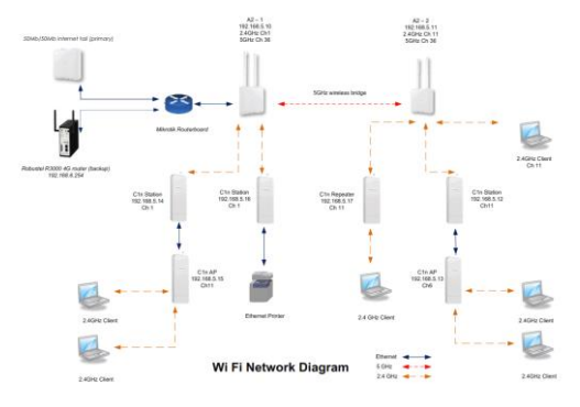
Integrated Altai A2 & C1n with a 4G router to provide a quick WiFi solution for one-off event
