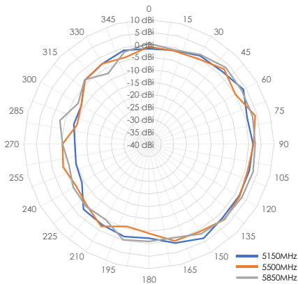
5 GHz XY Plane
