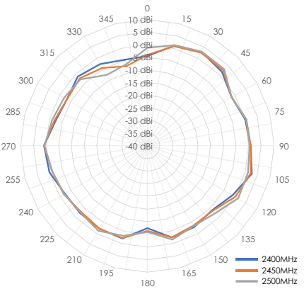
2.4 GHz YZ Plane
