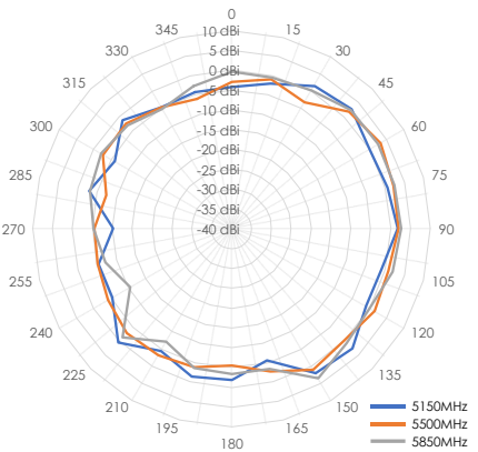
5 GHz YZ Plane
