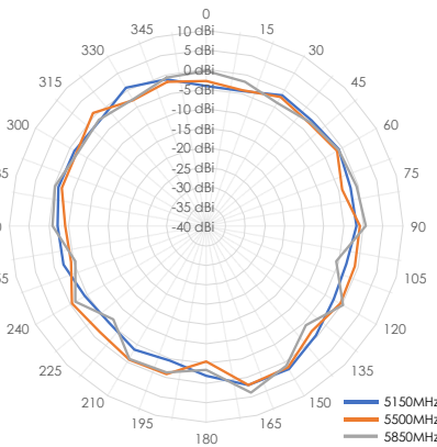
5 GHz XZ Plane
