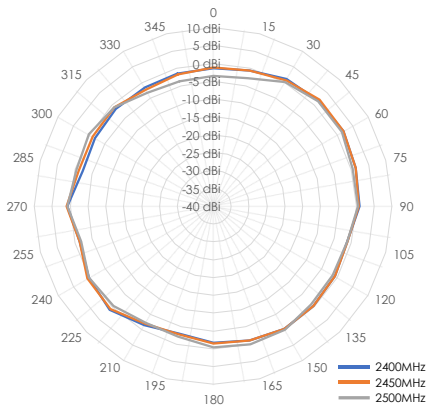
2.4 GHz XY Plane
