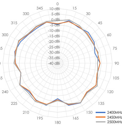
2.4 GHz XZ Plane
